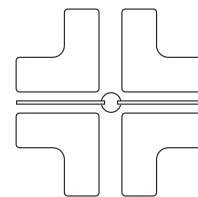
Shared Cable Trays in Centre Position (2 Way) (No Screens/Brackets)
